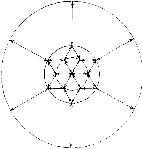
Pattern of electron field cavity wave resonance
